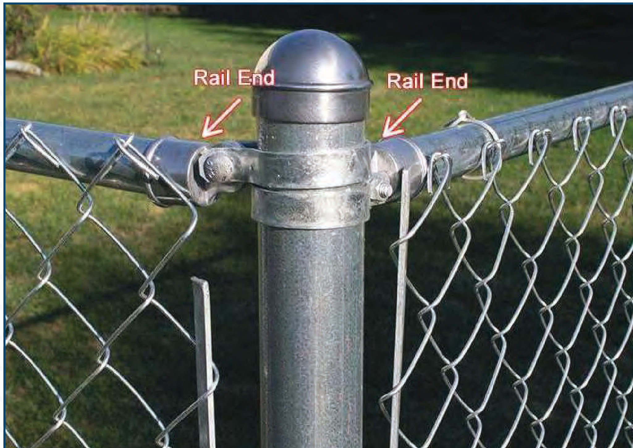
Rail end fix the horizontal post
