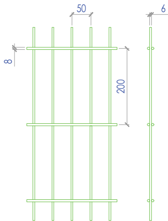
MESH DETAIL
