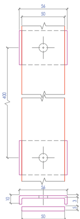
FIXING CLAMP DETAIL OPTION 1
