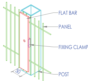
ISOMETRIC VIEW OPTION 2
