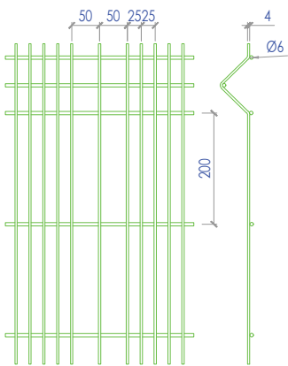
MESH DETAIL SCALE: 1:10MTRS
