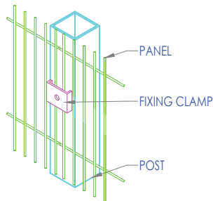
ISOMETRIC VIEW OPTION 1
