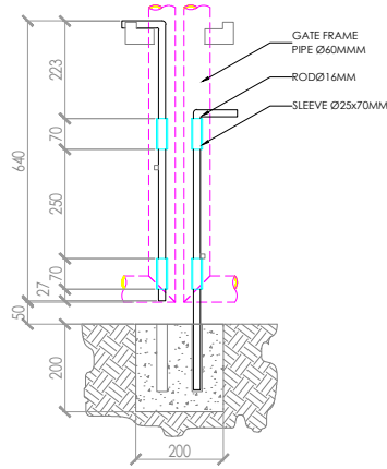
DROP BOLD DETAIL P - 603
