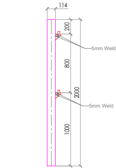
GATE POST P - 601
