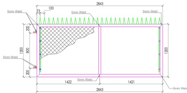
GATE FRAME WELDING ASSEMBLY P - 602
