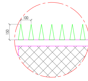
C SPIKES DETAIL
