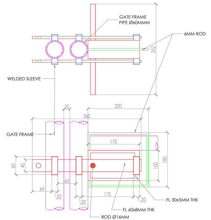
LOCK DETAIL
