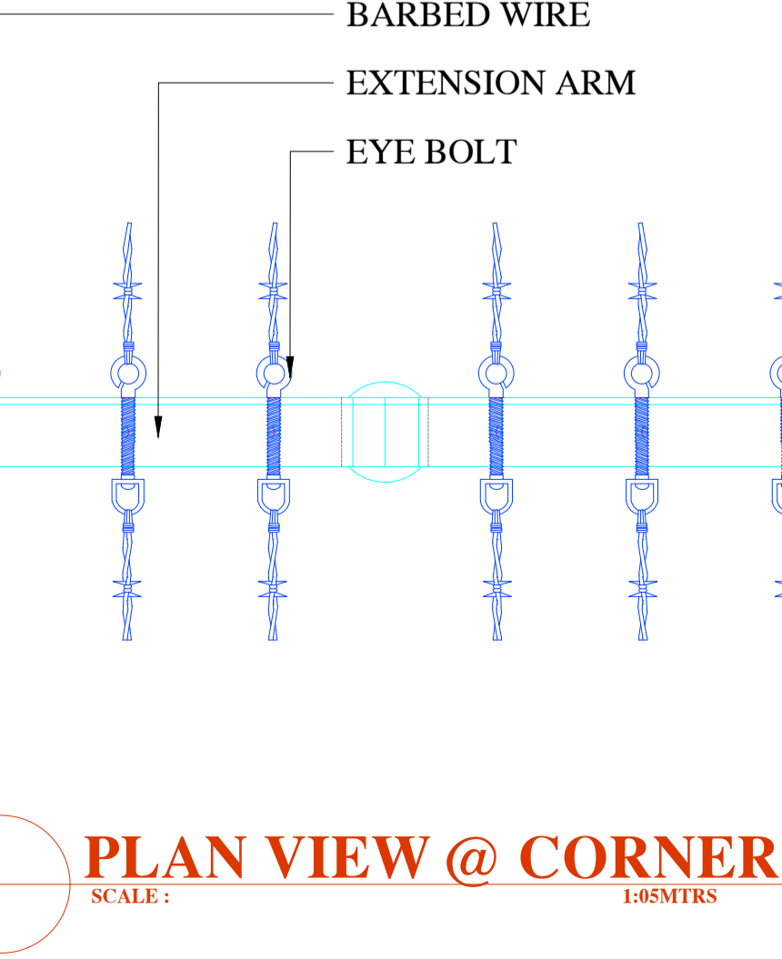
DETAIL 05 SCALE: 1:05MTRS
