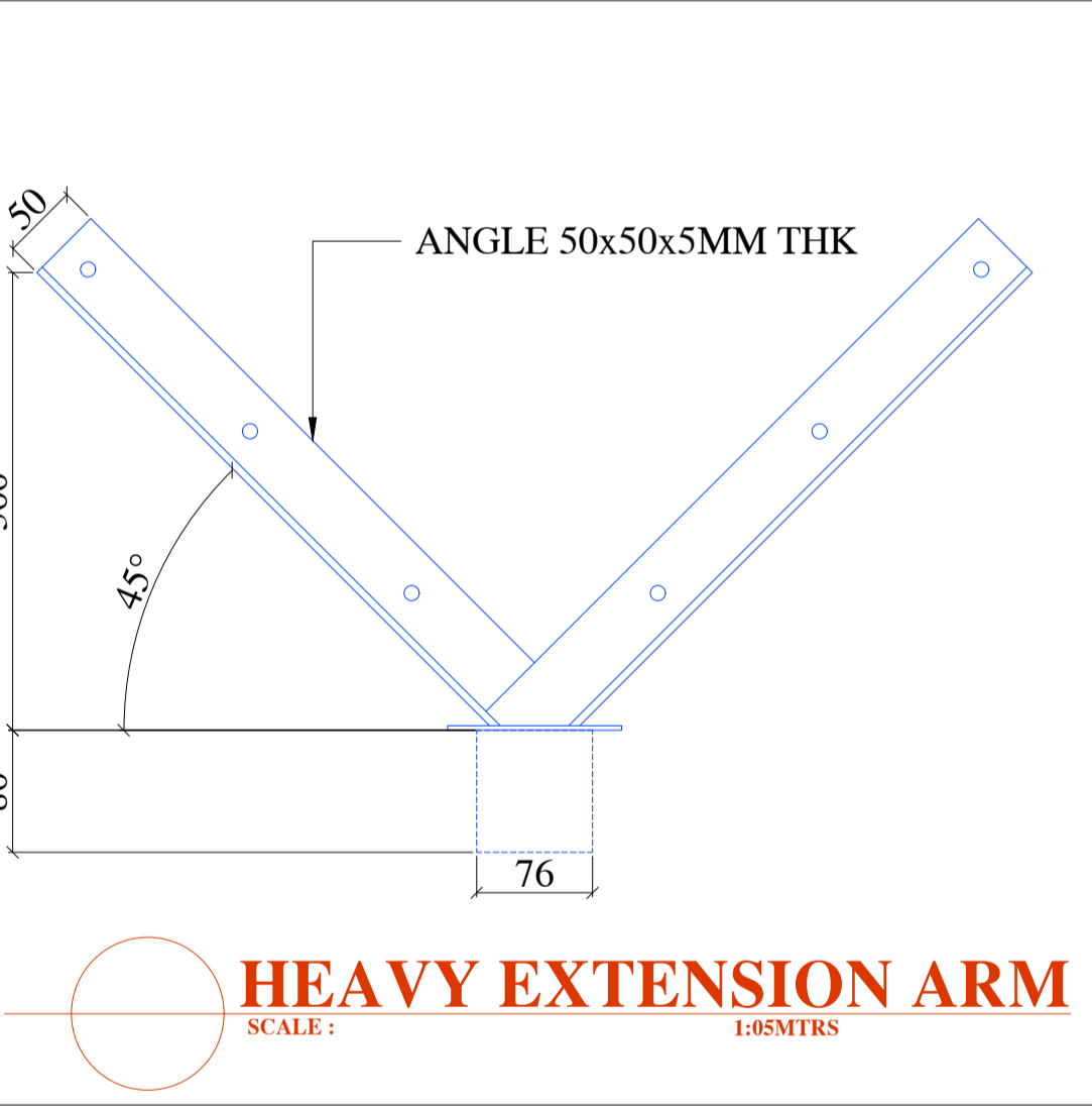
DETAIL 01 SCALE: 1:05MTRS
