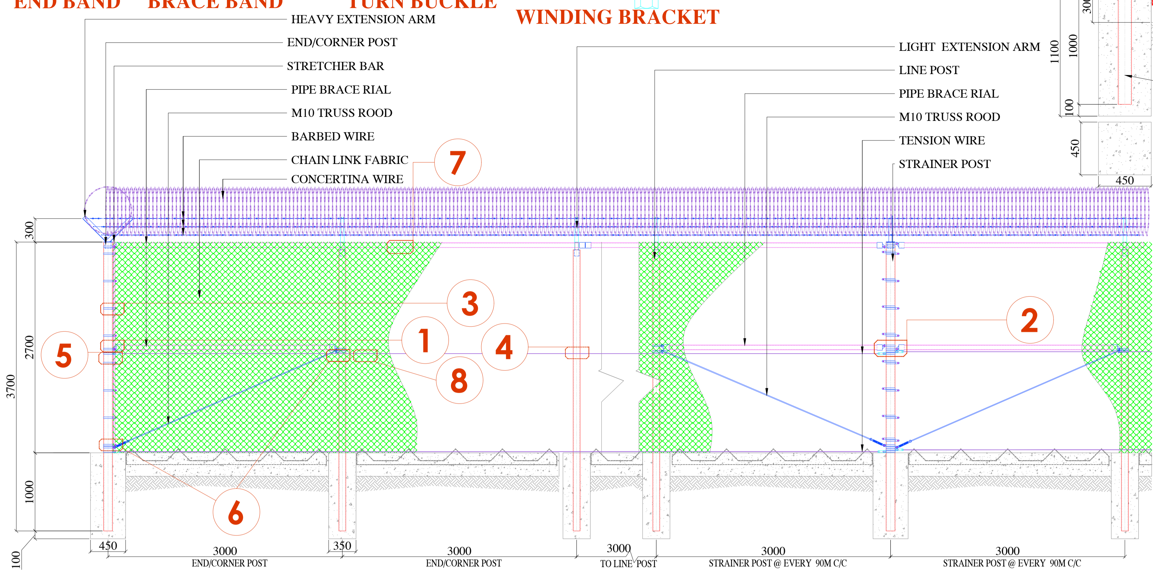
TYPICAL ELEVATION SCALE: 1:25MTRS
