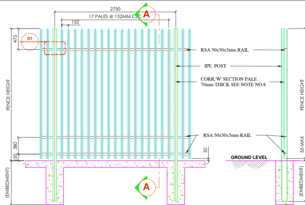
TYPICAL HIGH PALISADE FENCE
