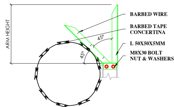
EXTENSION ARM DETAIL
