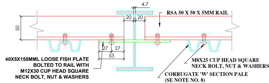
02 CONNECTION DETAIL
