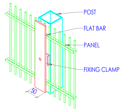
ISOMETRIC VIEW OPTION 2
