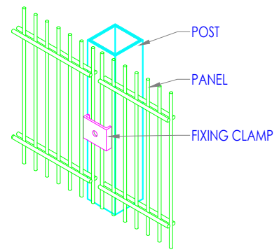
ISOMETRIC VIEW OPTION 1
