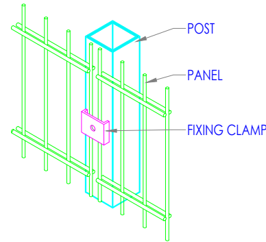
ISOMETRIC VIEW OPTION 1
