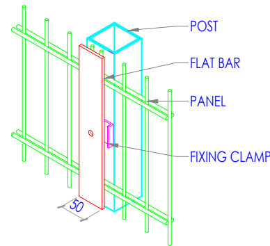
ISOMETRIC VIEW OPTION 2
