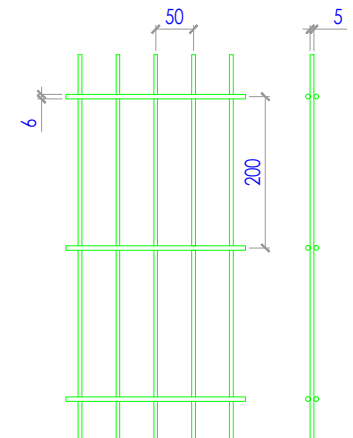
MESH DETAIL SCALE: 1:10MTRS
