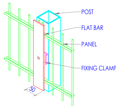
ISOMETRIC VIEW OPTION 2
