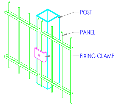
ISOMETRIC VIEW OPTION 1
