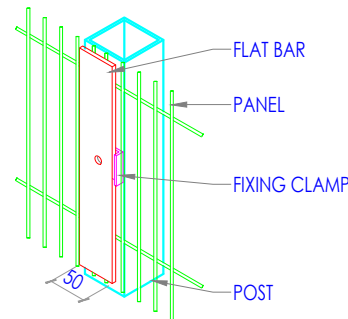
ISOMETRIC VIEW OPTION 2
