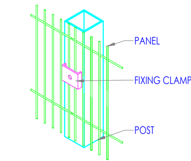
ISOMETRIC VIEW OPTION 1
