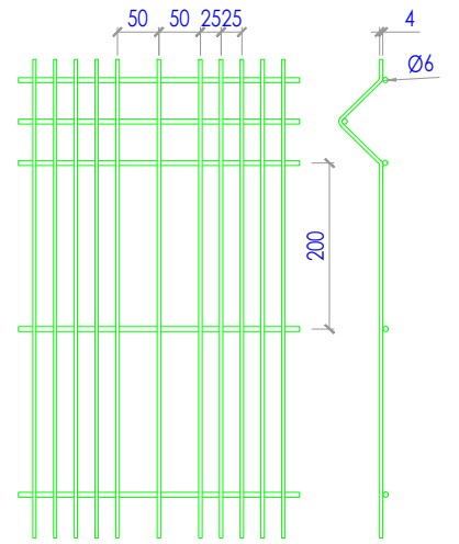
MESH DETAIL SCALE: 1:10MTRS
