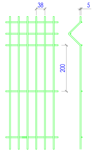
MESH DETAIL SCALE: 1:10MTRS
