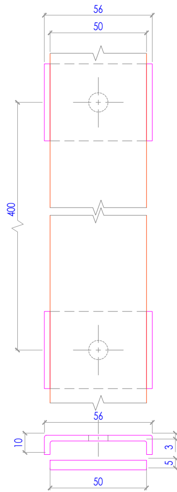
FIXING CLAMP DETAIL OPTION 2
