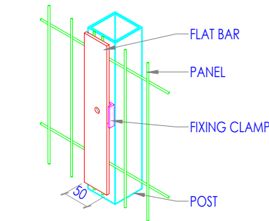
ISOMETRIC VIEW OPTION 2
